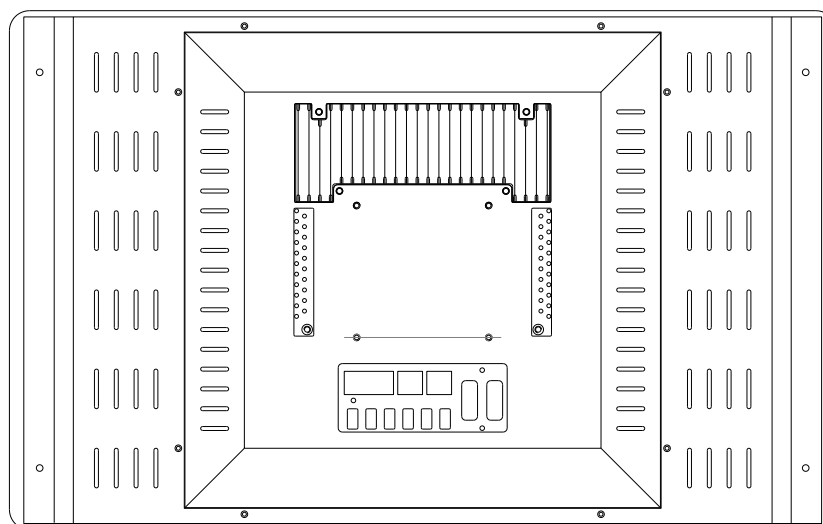
Figure 6: rear view
