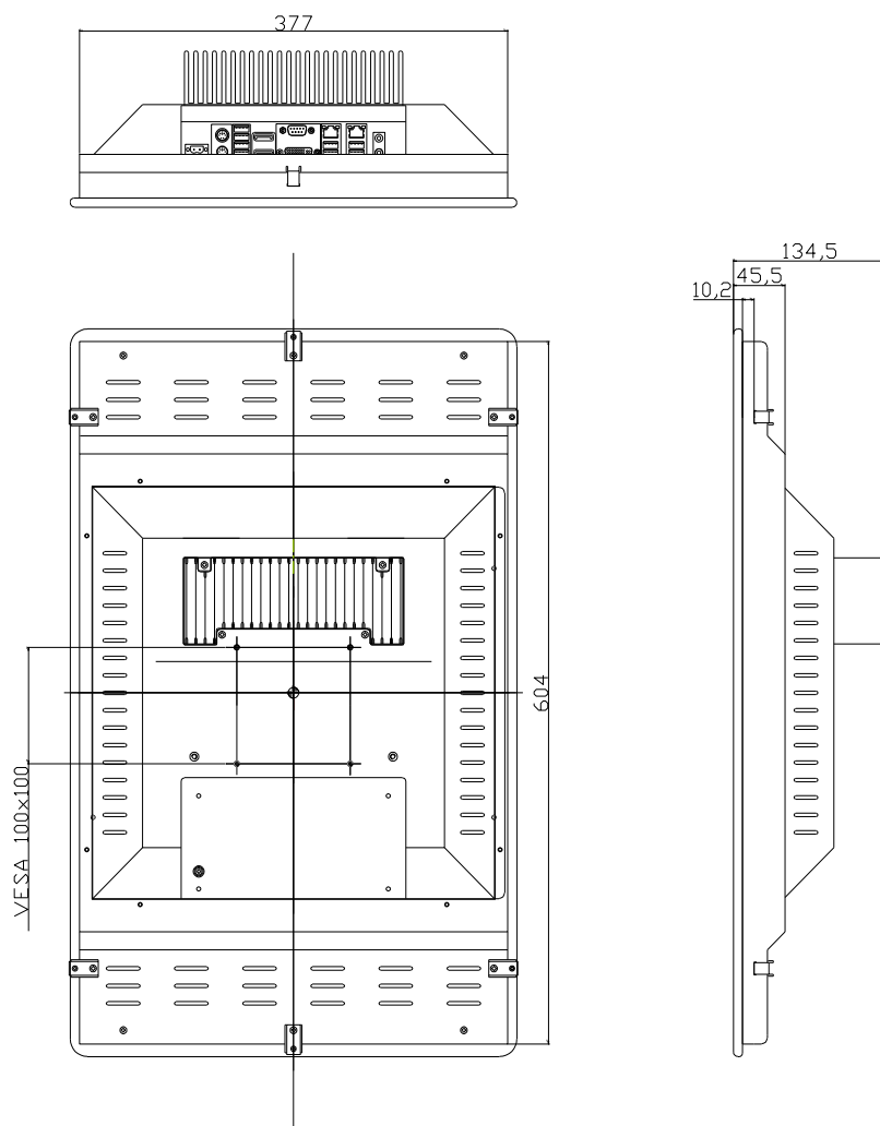
Figure 4: rear view
