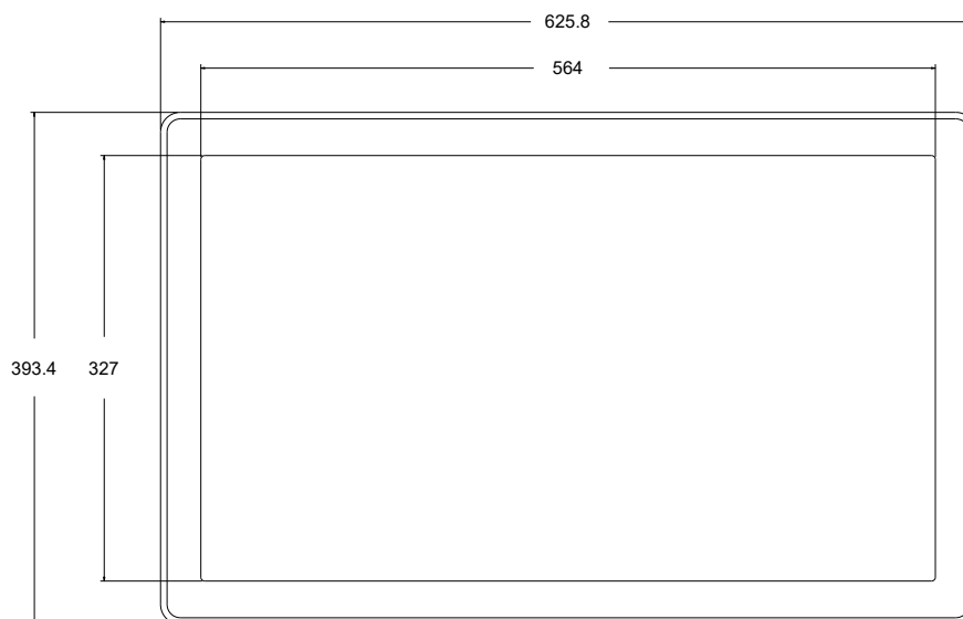
Figure 5: Front View
