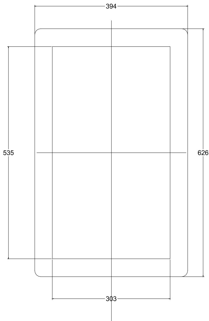
Figure 3: Front View
